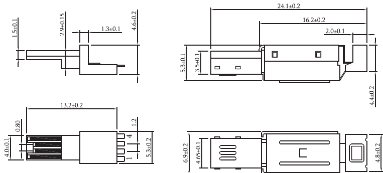
Part No.:MUSB-M4S-BB-L
